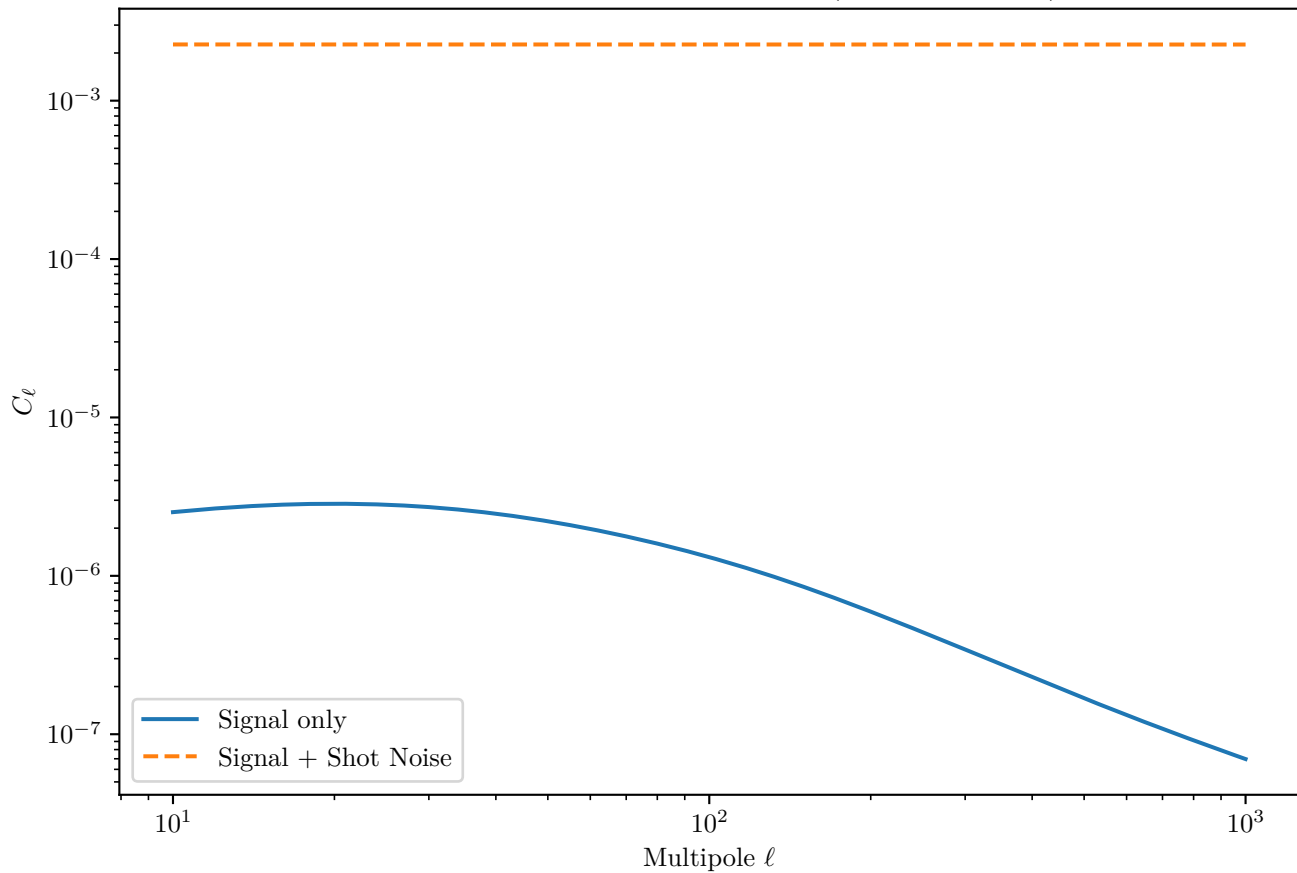
FRB Auto-Correlation Angular Power Spectrum (Shallow Survey) for Magnetars
